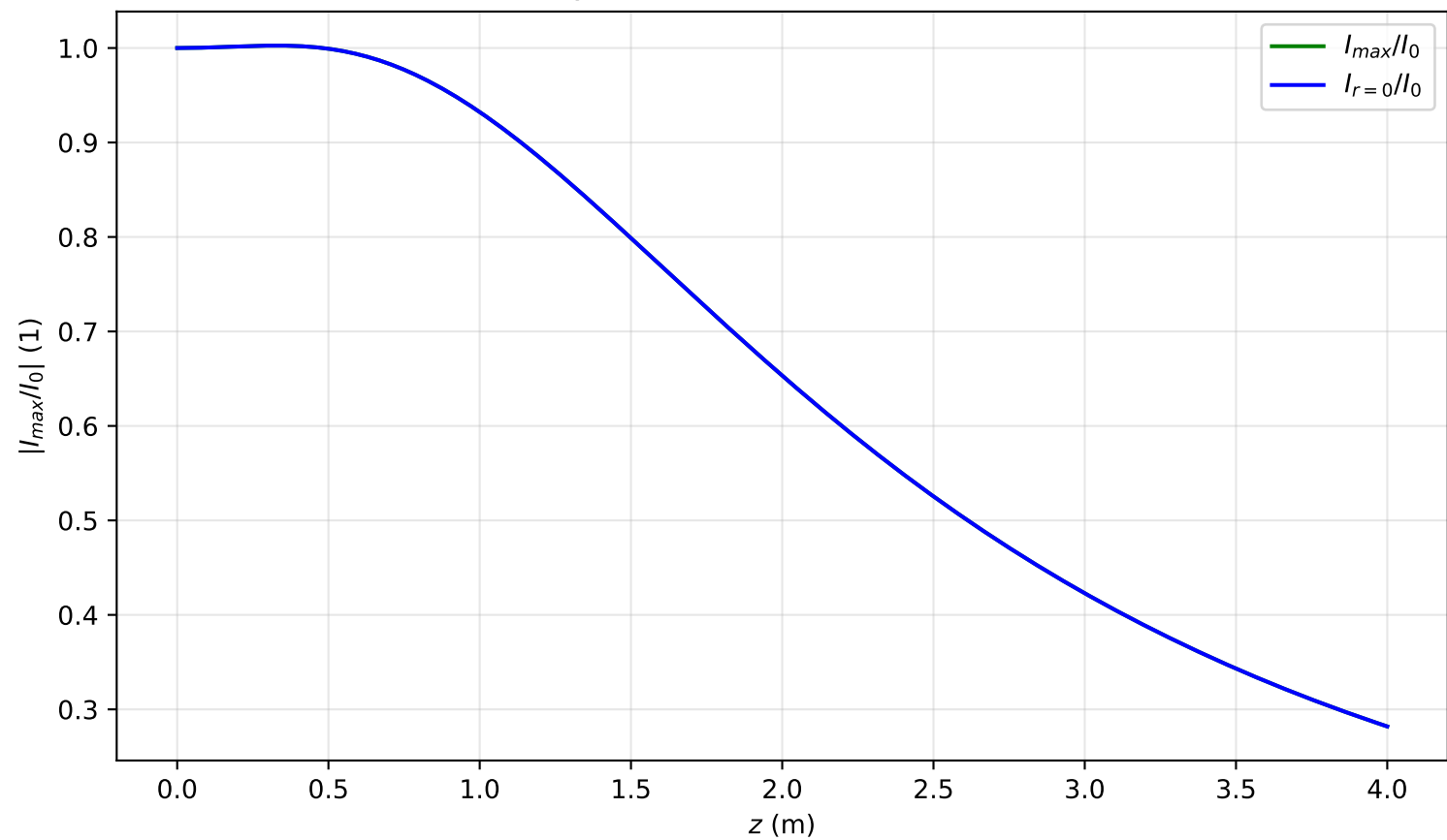
I_{max}(x = 0, y = 0, z)/I_0 , P_{in}=0.3P_{cr} , artificial time
